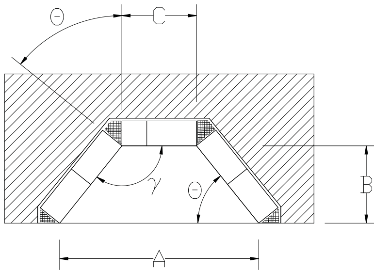
Figure 3. Hearth--Plan View
