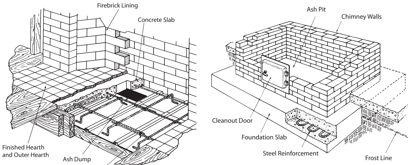
Figure 2. Examples of Typical Foundation Construction
