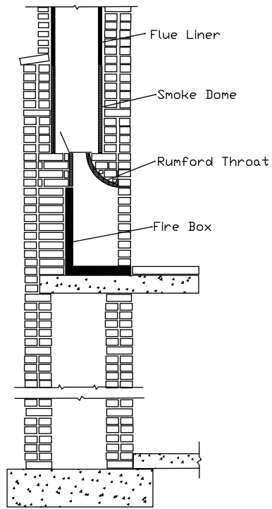
Figure 1. Side Cross Section of a Rumford Fireplace
