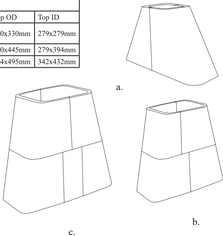
Figure 14. Smoke Dome Sections for a.) 30" & 36" Rumford--2 pieces, b.) 42" Rumford--4 pieces and c.) 48" Rumford--6 pieces.
